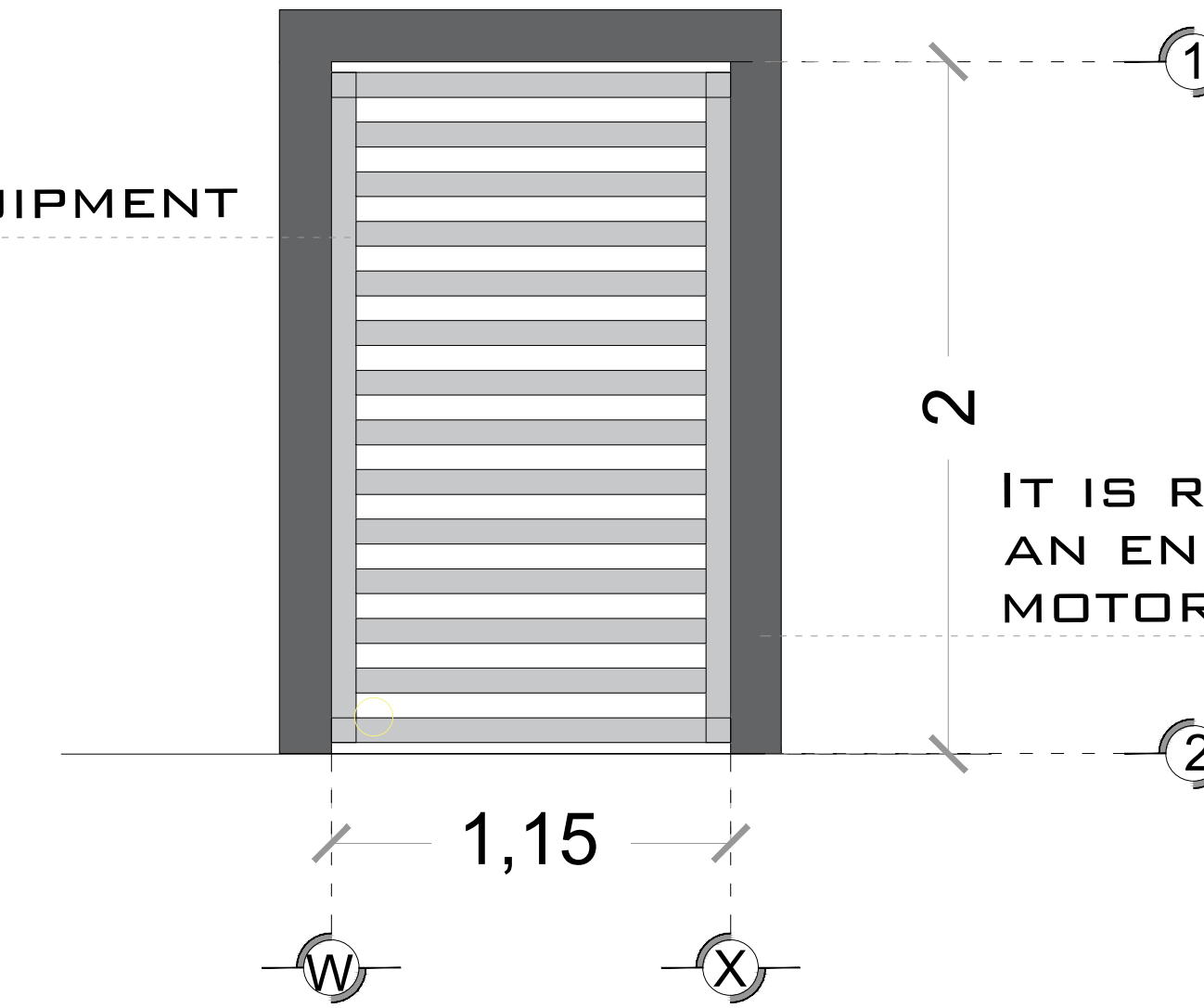
DESCRIPTION OF HYDRAULIC UNIT CABINET (FRONT VIEW)
