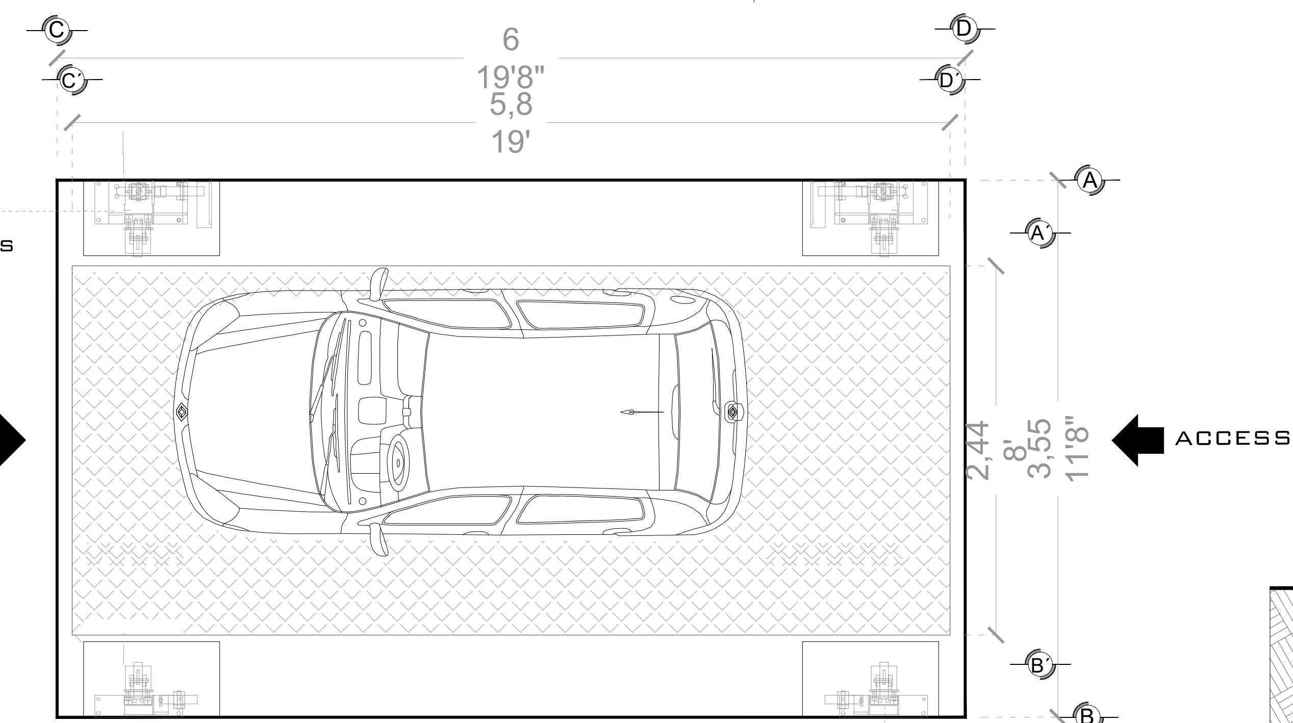
CAR LIFT FRONTAL
