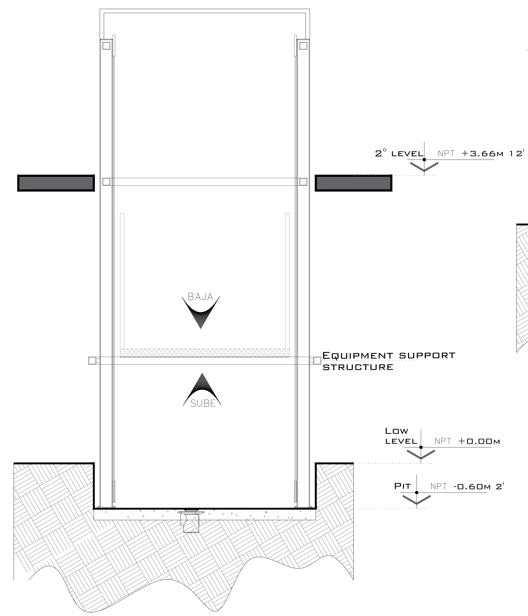
CAR LIFT FRONTAL
