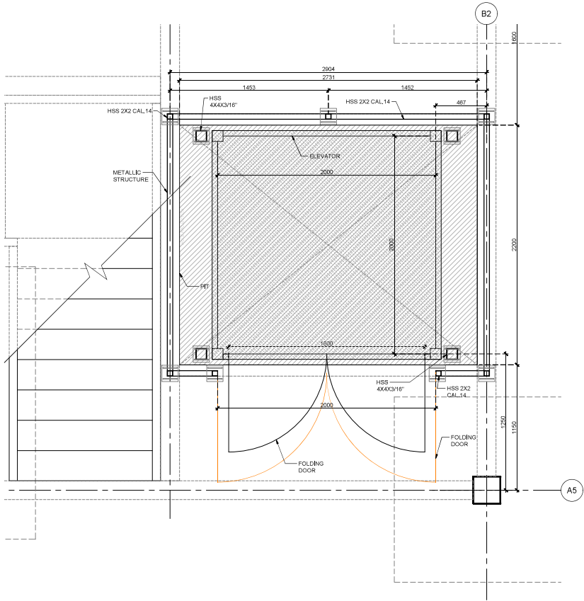
LIFT PLAN
