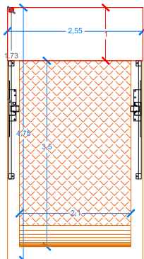
RAMPA LIBRE 2.10M x 3.50M
