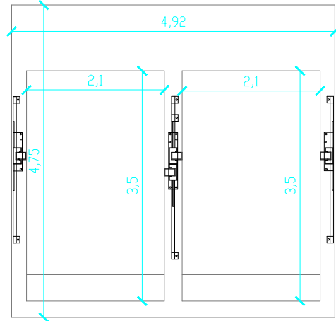
RAMPA TR EVOLUTION 2.10M X 3.50M
