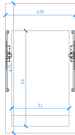
RAMPA TR EVOLUTION 2.10M X 3.50M
