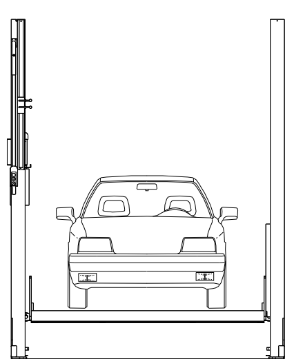
VISTA FRONTAL
